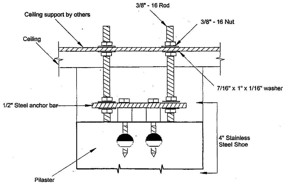
CEILING CONNECTION
