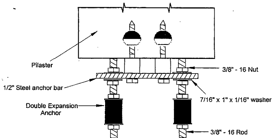
FLOOR CONNECTION
